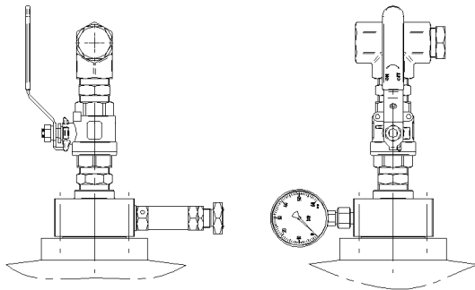
S/ens. tête de bouteille Receiver head sub set 1:5
